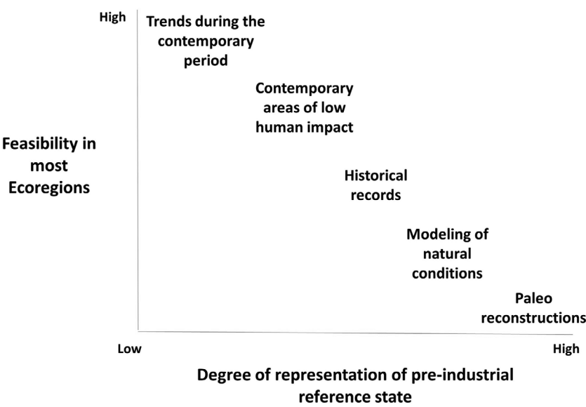
FIGURE 3 Various methods of establishing reference state for ecosystem integrity. These are expressed along gradients of degree of representation of the natural reference state and feasibility of implementing the method in most contemporary ecosystems
