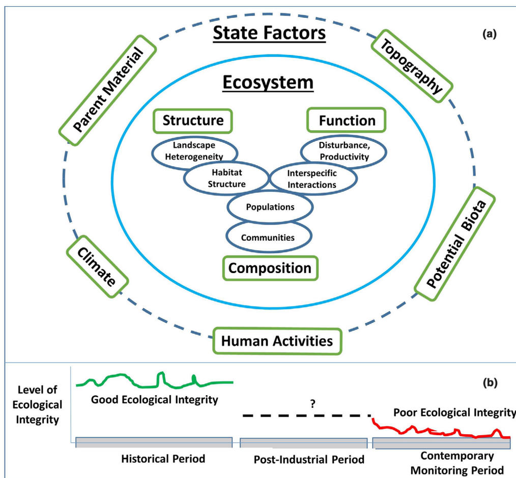
FIGURE 2 Representation of the concept of ecosystem integrity in the context of the ecosystem and controlling state factors. (A) An ecosystem is characterized by its structure, function, and composition as influenced by broad-scale state factors such as climate. (B) Ecosystem integrity represents the condition of elements of ecosystem structure, function, and composition in the current period relative to that characteristic of the ecosystem prior to modern human influence. The trend line depicts declines in ecosystem integrity during a contemporary monitoring period
