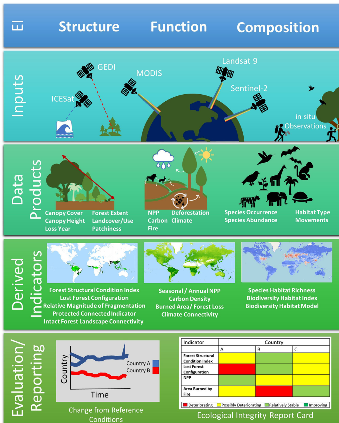
FIGURE 1 Flow diagram of the recommended approach for tracking indicators of ecosystem integrity
